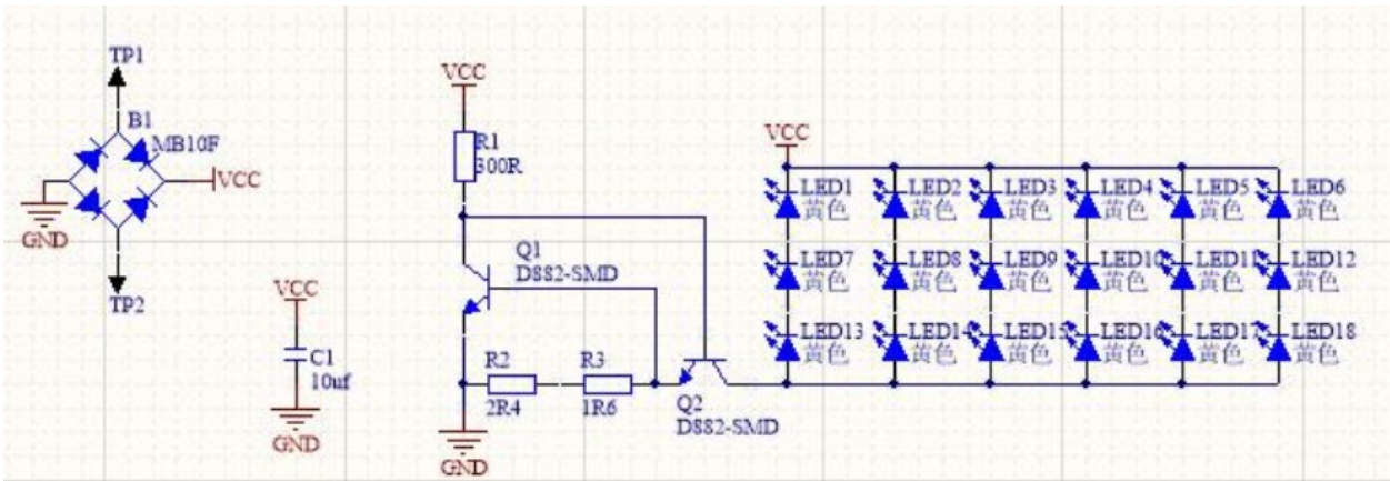
12V/1.8W, Non-replaceable light source
