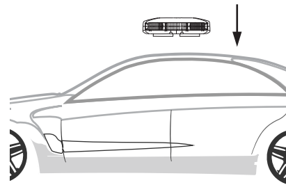
Installed by magnet at the top of car
