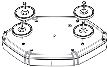
Four magnets were fixed with 4 screws at the bottom of the lightbar
